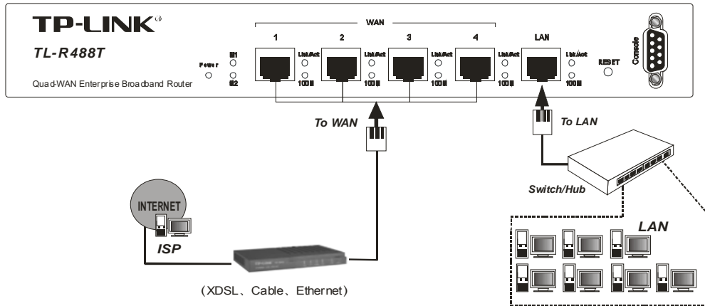
Figure 3-1 Hardware Installation of the TL-R488T Load Balance Broadband Router
